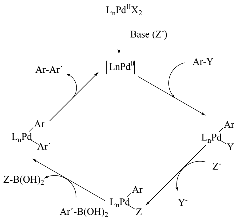
Figura.1.8.1.1 Mecanismo Suzuki-Miyaura
