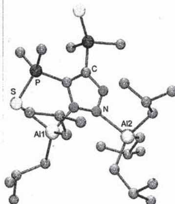
Figure 9. Molecular structure of compound 13 .
