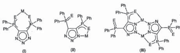
Figure 1. Coordination modes reported for ligands 1–3.
