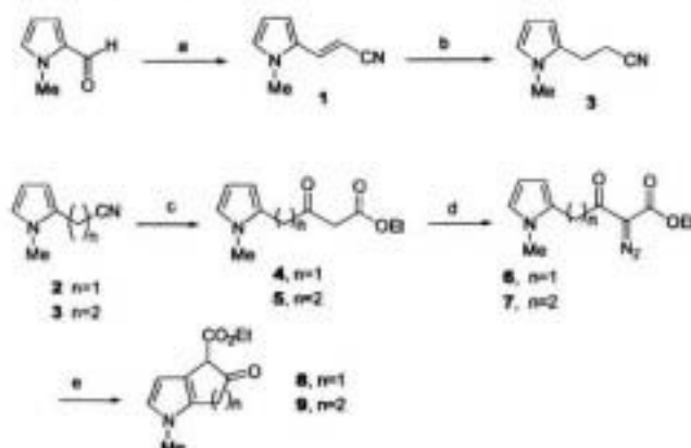
Scheme 1. Reagents and conditions: (a) \text{Ph}_3\text{PCyCN} , toluene/ \text{CH}_2\text{Cl}_2 , reflux, 36 h; (b) \text{H}_2 , Pd/C, MeOH, RT, 6 h; (c) \text{BrCH}_2\text{CO}_2\text{Et} , Zn, THF, reflux, 8 h; (d) \text{TsN}_3 , \text{Et}_3\text{N} , \text{CH}_2\text{Cl}_2 , RT, 12 h; (e) \text{Rh}_2(\text{OAc})_4 , \text{ClCH}_2\text{CH}_2\text{Cl} , reflux, 3 h.
