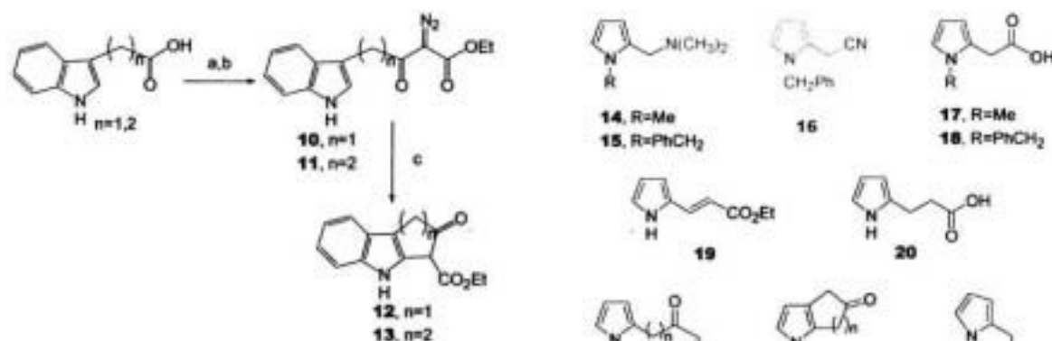
Scheme 2. Reagents and conditions: (a) oxalyl chloride, DMAP, THF, -65\text{ }^\circ\text{C} , 30 min; (b) ethyl diazoacetate, \text{Et}_3\text{N} , -65\text{ }^\circ\text{C} for 30 min and 12 h at RT; (c) \text{Rh}_2(\text{OAc})_4 , \text{ClCH}_2\text{CH}_2\text{Cl} , reflux, 3 h.
