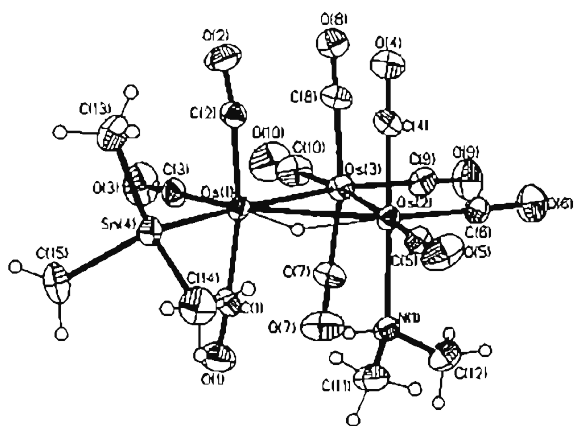
Figure 1. Molecular structure of 5 with the atom-numbering scheme.
